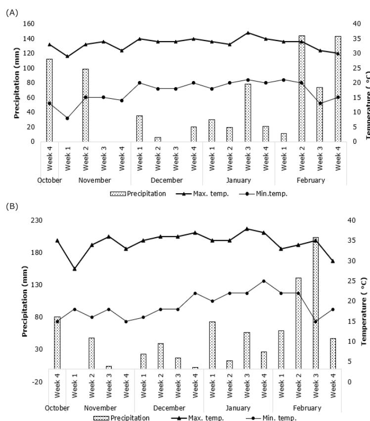
Figure 1. Precipitation, maximum and minimum temperatures during the growing period of sesame in Saltos del Guairá (A) and Ybyrarobana (B). 2022/23.
